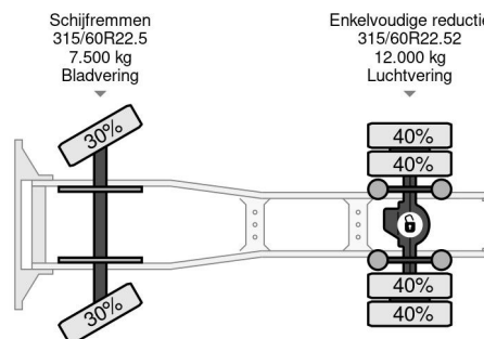
Mercedes-Benz Actros 1842 4X2 - EURO 5 + FULL SPOILER
