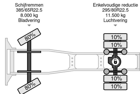
DAF XF 460 4X2 EURO 6 SKIRTS AUTOMATIC
