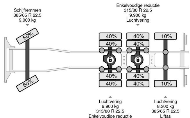
Scania S580 V8 NGS 8X4*4 EURO 6
