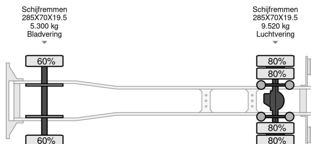
Iveco ML 150 -220, DHOLLANDIA LIFT, BOX 760X250... 4x2
