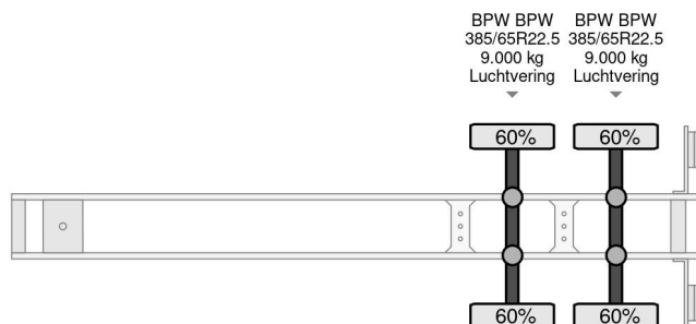
Groenewegen DRO-14-18 - 2 AXLE BPW
