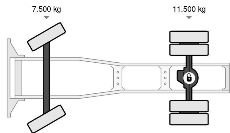
DAF XF 480 4X2 - EURO 6 + TIK IN MOTOR
