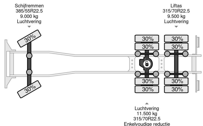
Scania R580 V8 6X2 VDL HOOK 20T RETARDER EURO 6 2...
