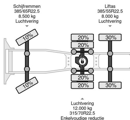
MAN TGX 26.500 6X2 - EURO 6 + LIFTING AXLE
