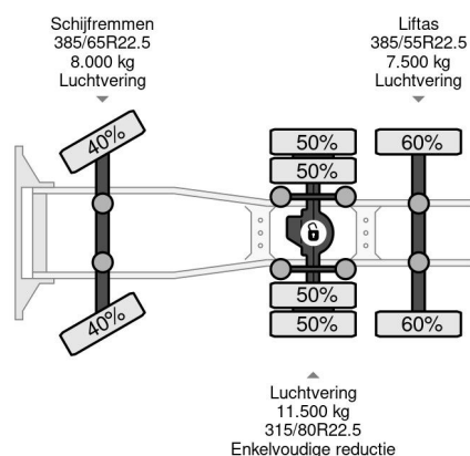
Scania S500 6X2 - EURO 6 + LIFT AXLE
