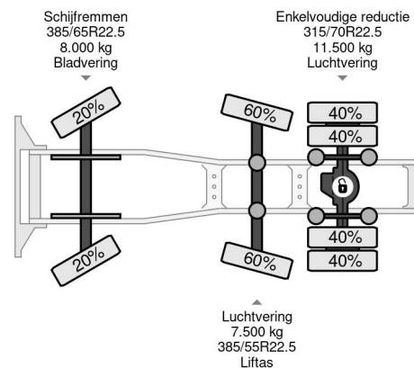
DAF XF 480 6X2 - EURO 6 + LIFT/STEERING AXLE + FULL...
