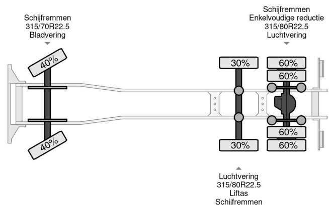
Scania R420 6X2 MULTILIFT SLT 180
