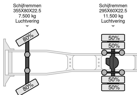
Volvo FH FH420
