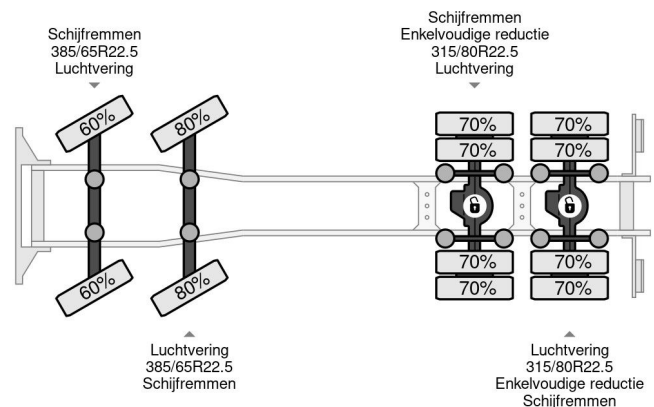
Volvo FH 500 8X4 EURO 5 + HIAB 232 HIPRO 2018 + REM...
