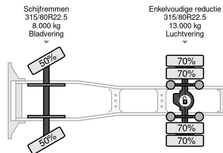
DAF XF 460 4X2 - EURO 6 + NL TRUCK + TÜV 08-2025
