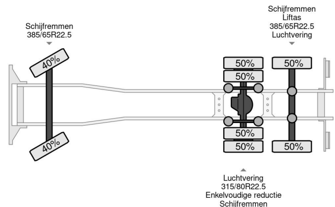
Volvo FMX 410 6X2 EURO 6 HIAB 18T HOOK + HIAB 144 + ...
