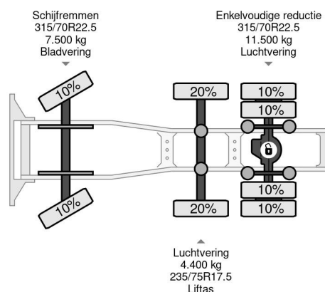
DAF XF 105.460 6X2 - EURO 5 + LIFTING AXLE
