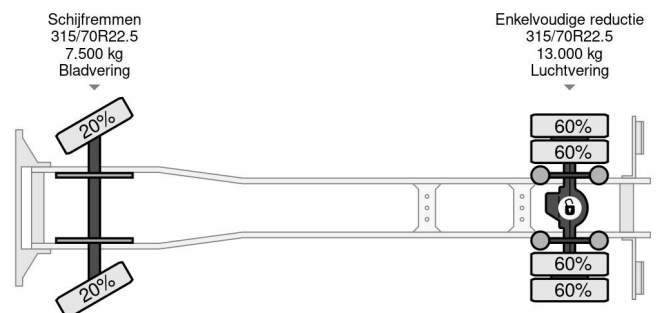
DAF CF 290 4X2 - EURO 6 + HEATING SYSTEM + BÄR CA...
