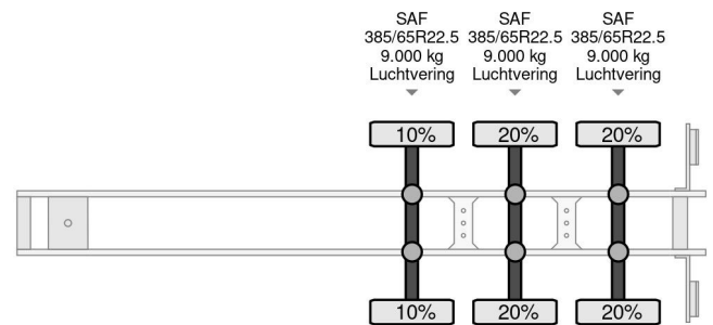
Krone SD - CARRIER VECTOR 1850 + 3X SAF AXLE + LIFT...
