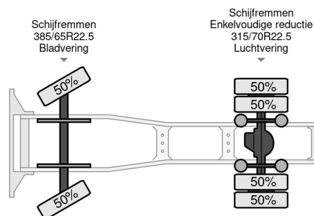
Volvo FH 460 4X2 SKIRTS EURO 6 2019
