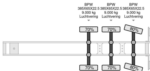
Sor 3 AXLE - ISOLATED BOX (WITHOUT FRIGO UNIT!) + L...
