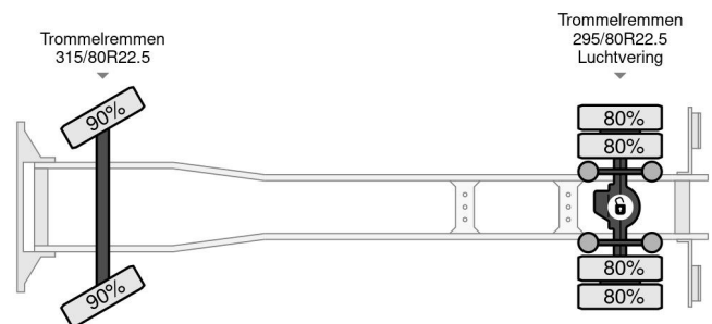
Volvo FM 7.290 4X2 EURO 2 + PM 22SP5 + REMOTE CON...
