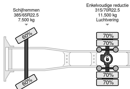
Scania R450 4X2 EURO 6 + ADR + APK 02-2025
