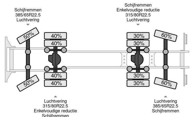
Volvo FH 460 8X4 HIAB 211 BJ 2016 + REMOTE CONTROL...
