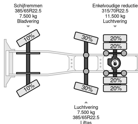
Scania R450 6X2 EURO 6 STEERING AXLE
