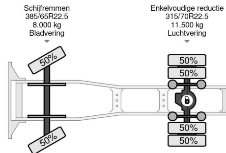
DAF XF 460 4X2 EURO 6 RETARDER SKIRTS
