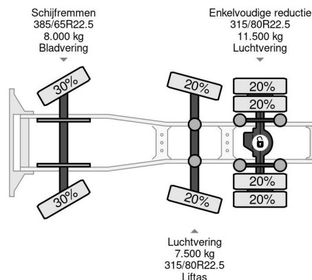
Volvo FH 480 6X2 EURO 5 + HYDRAULICS + STEERING AXLE
