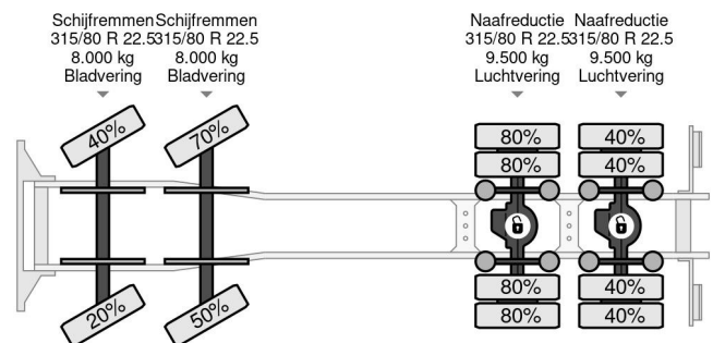
Volvo FM 410 8X4 MIXER 9m3 + LIEBHERR CONVEYOR BELT
