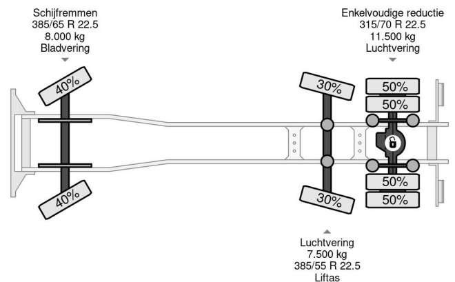
Volvo FM 370 6X2 EURO 5 HIAB 144E-5 + REMOTE
