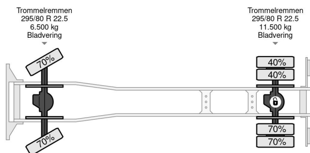
DAF 1900 TURBO 4X4 HOOKLIFT
