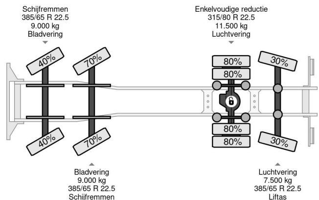
Scania R490 8X2 EURO 6 + EFFER 1750/4S + REMOTE
