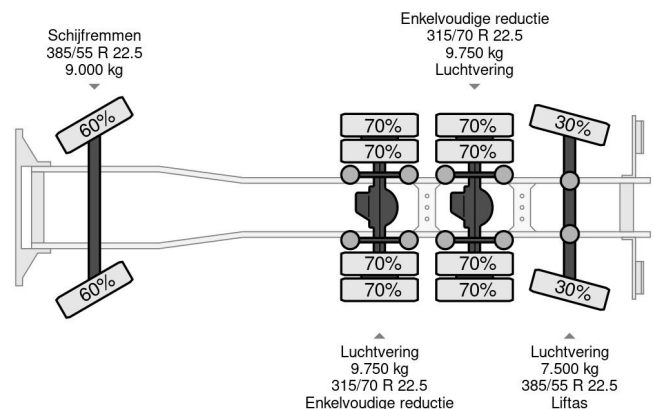
Volvo FH 16.750 8x4 CHASSIS - i-Shift
