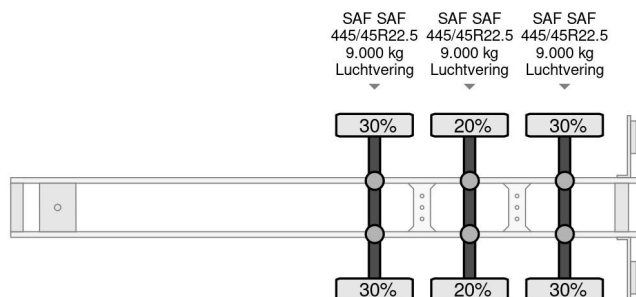
Schmitz Cargobull SCS 24/L - 3 AXLE SAF MEGA
