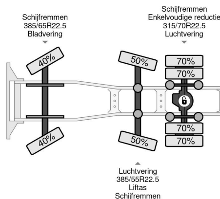
Volvo FH 460 6X2 PALFINGER 2300 + REMOTE CONTROL
