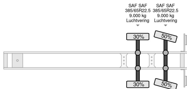
System Trailer TFSH 18 TRPLY - 2 AXLE SAF + STEERING ...
