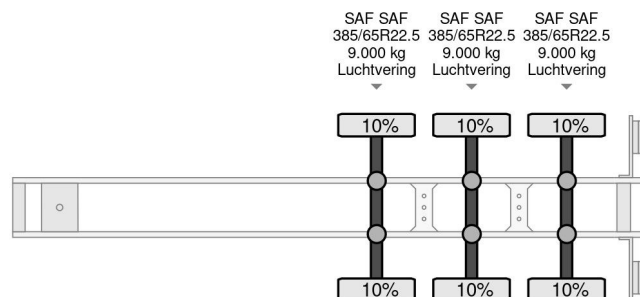
Broshuis 3 UCC-39/45 EU - 3 AXLE SAF + LIFTING AXLE
