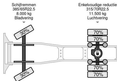
DAF XF 440 4X2 EURO 6 SKIRTS 2017
