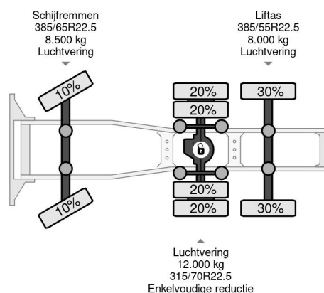
MAN TGX 26.500 6X2 - EURO 6 + LIFTING AXLE
