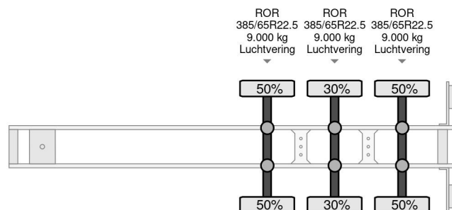
Atcomex 3 AXLE KIPPER BULK 1 COMP. 60.000 L
