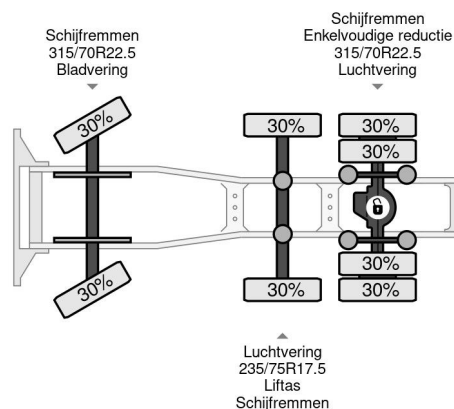
DAF XF 105.460 6X2 EURO 5 SKIRTS MANUAL GEAR HY...
