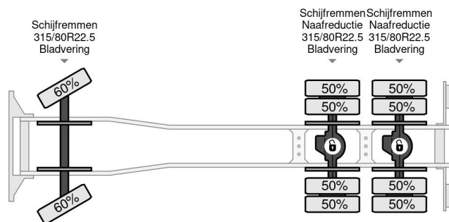
DAF CF 75.310 6X4 MANUAL GEAR EURO 3 FULL STEEL
