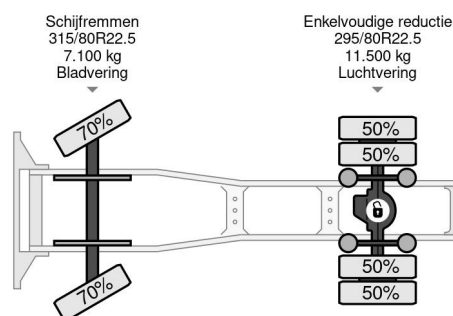
DAF CF 75.290 4X2 EURO 3 MANUAL GEAR
