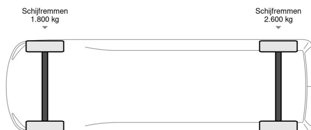
Iveco Daily 35C17 4X2 - EURO 5 + BUNK BU 7000 + CARRI...
