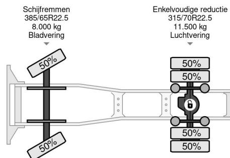
DAF XF 460 4X2 EURO 6 RETARDER SKIRTS
